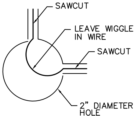
DETAIL "B"
