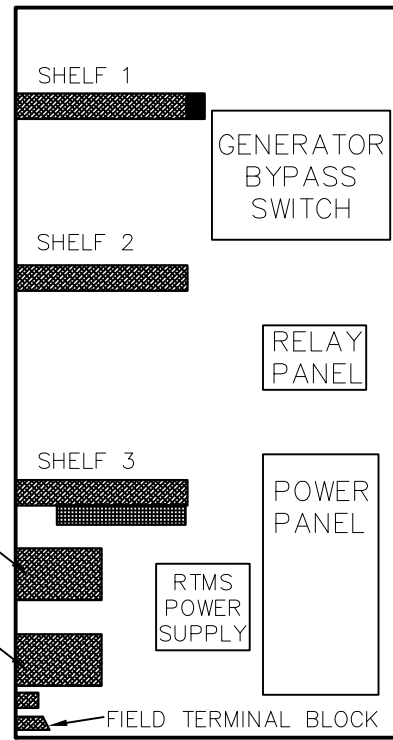
BOTTOM OF CABINET
