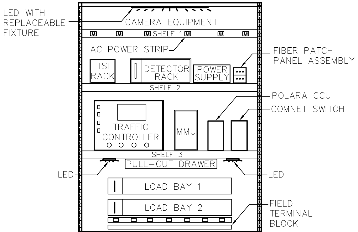
FRONT VIEW OF CABINET
